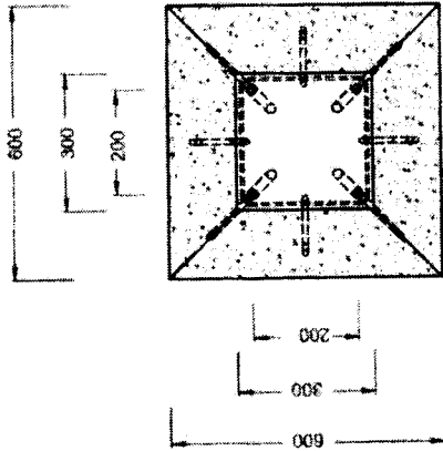
TOP VIEW SCALE 1:15
